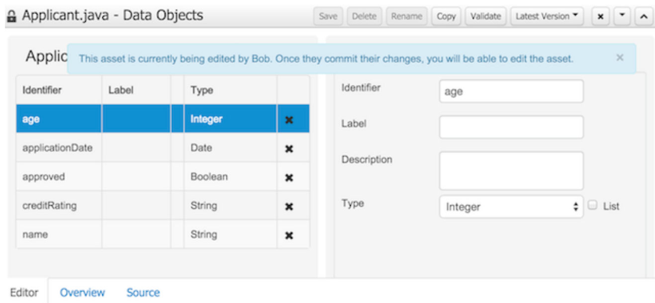
Figure 26.25. Locked assets cannot be edited by other users
