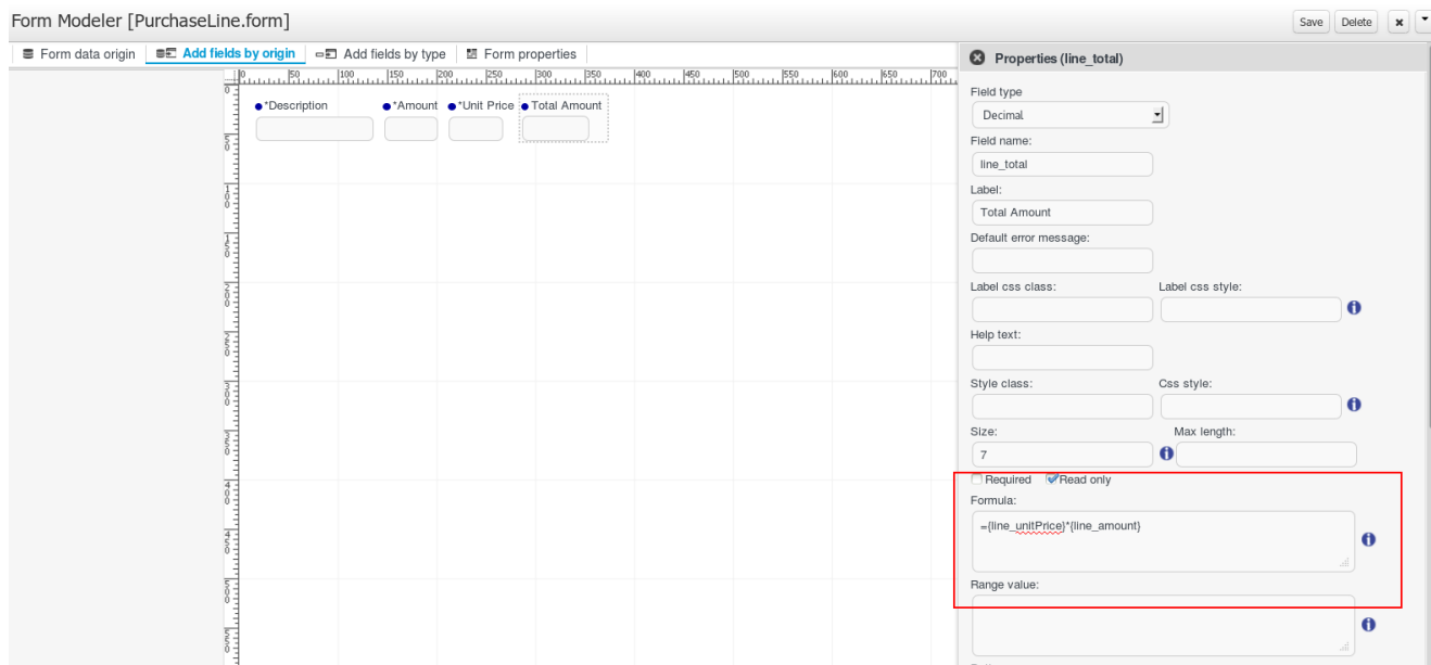
Figure 14.30. Rendering field with default formula
