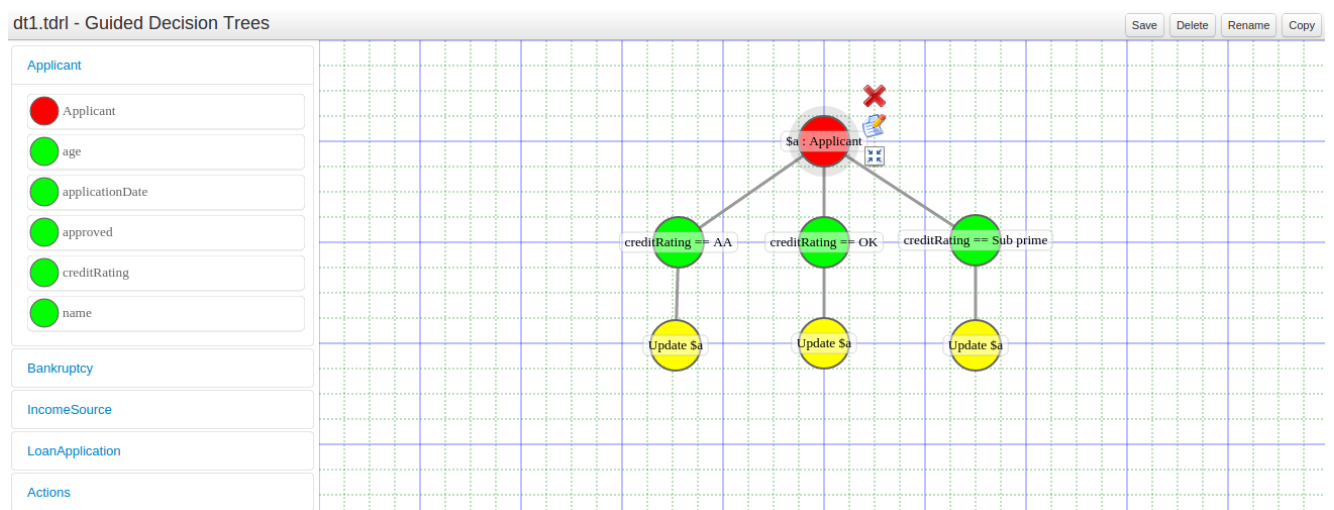
Figure 26.52. Example Guided Decision Tree
