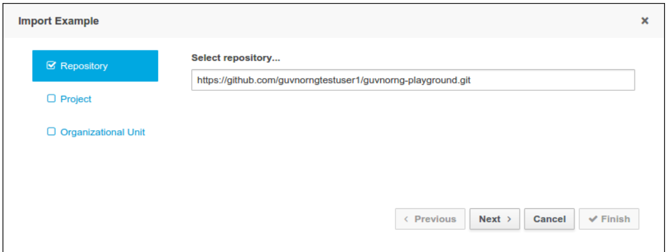
Figure 10.2. Import Examples - Wizard - Enter source Repository
