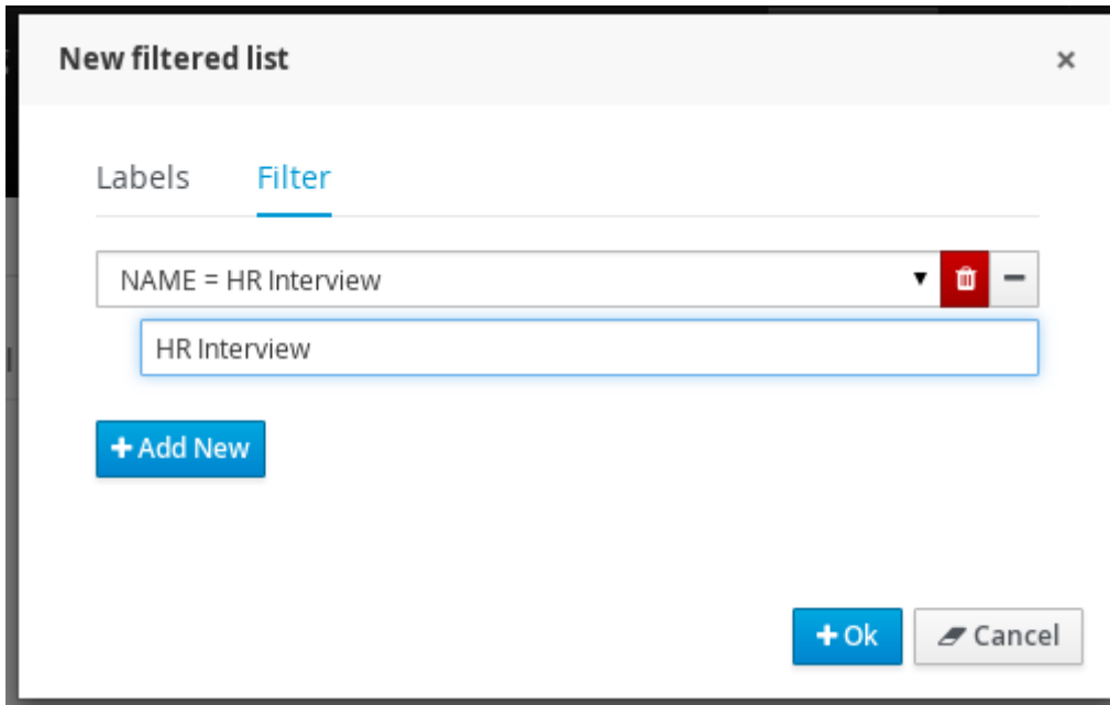
Figure 16.2. Filter by task name creation
