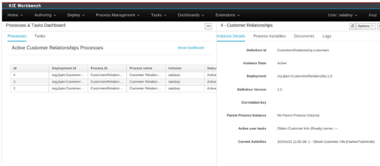
Figure 17.8. Task Dashboard
