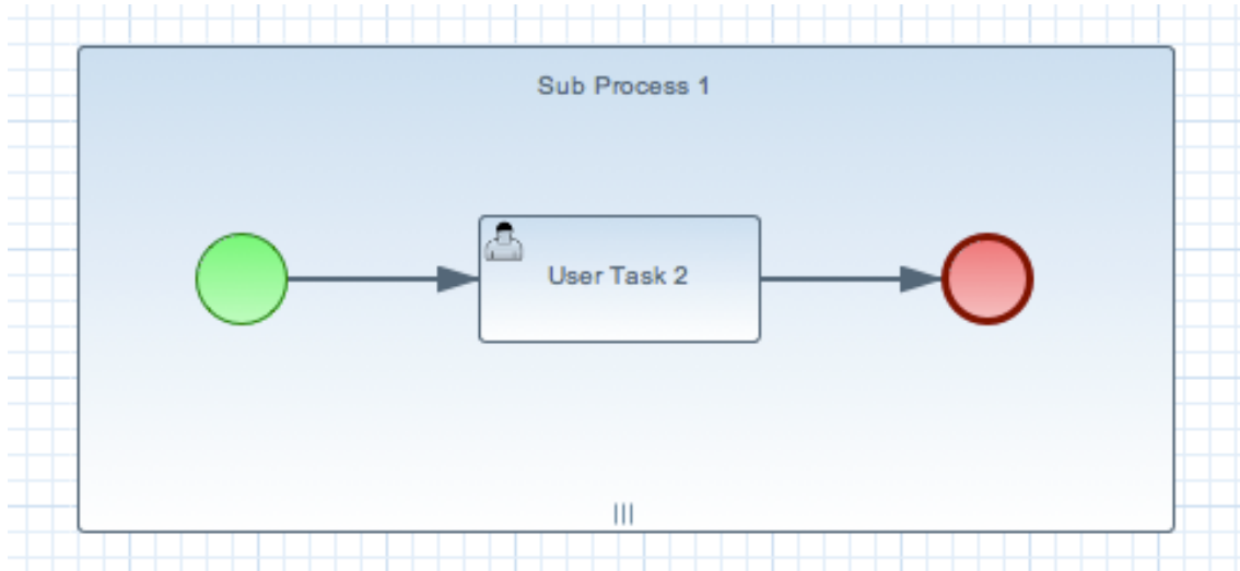
Figure 7.13. Multi-instance sub-process
