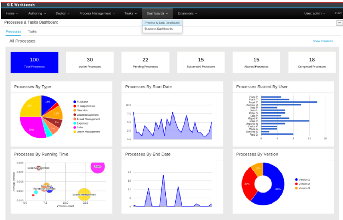
Figure 17.4. Processes dashboard
