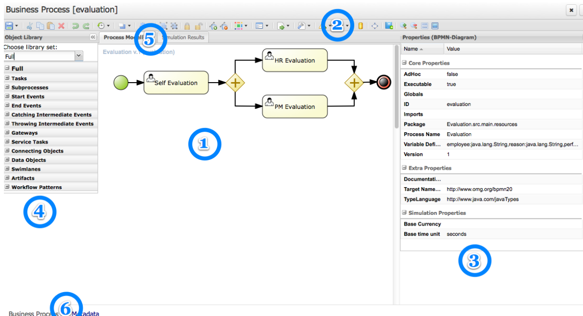
Figure 13.2. Designer sections
