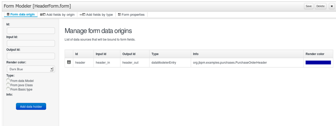
Figure 14.18. Data origin
