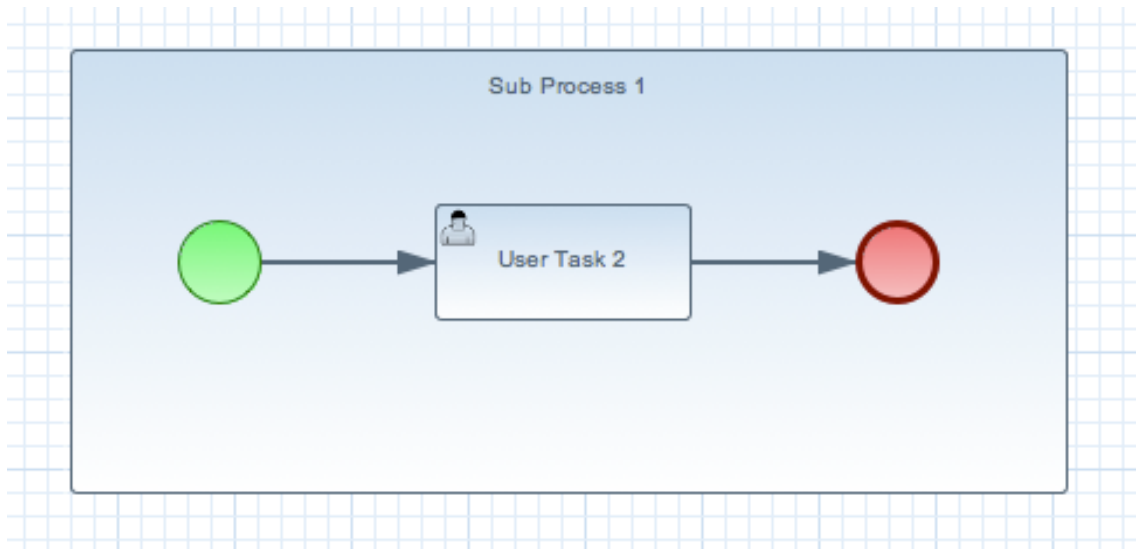
Figure 7.12. Embedded sub-process
