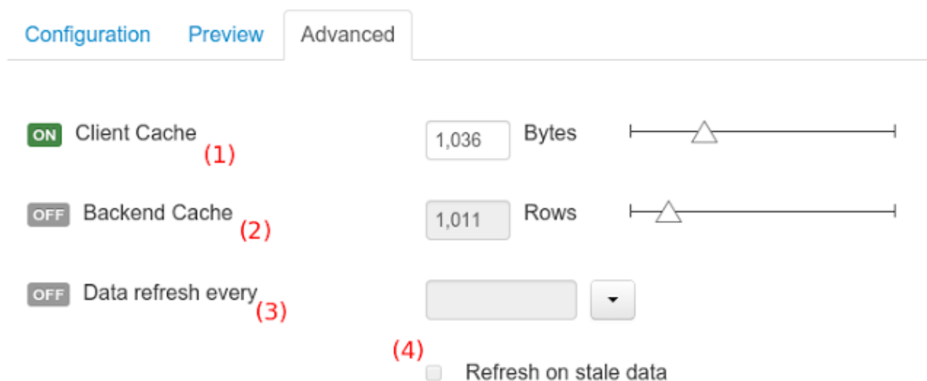
Figure 10.116. Advanced settings
