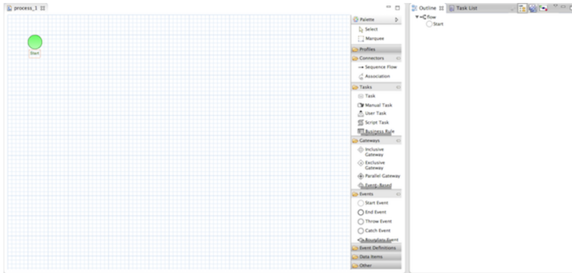
Figure 7.2. New process
