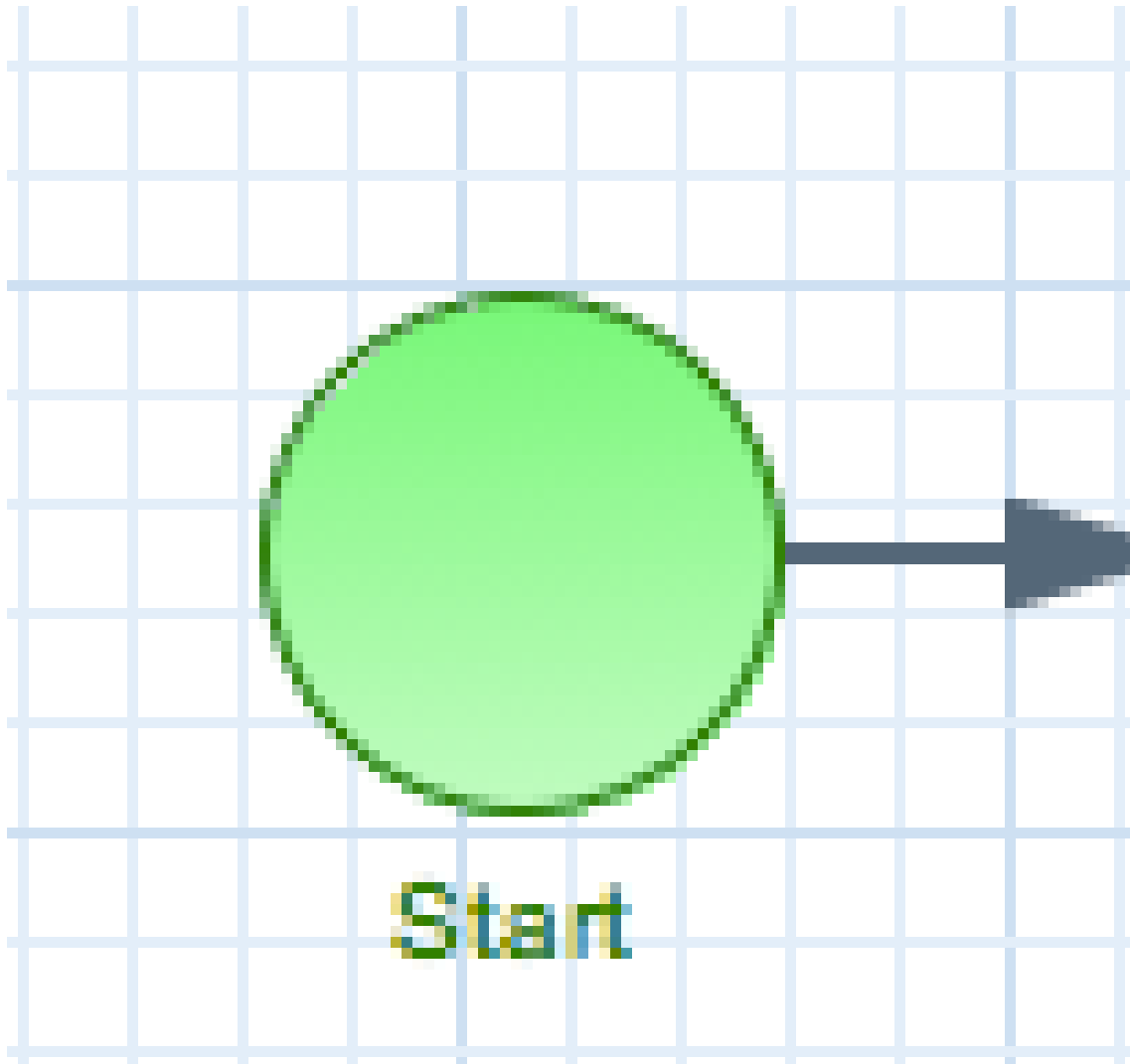
Figure 7.14. Start event
