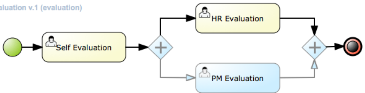
Figure 13.12. Locked Nodes
