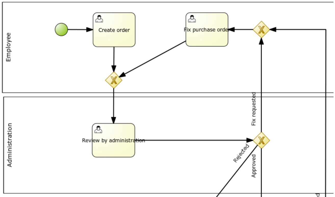
Figure 14.1. Process example
