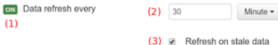
Figure 10.118. Refresh settings
