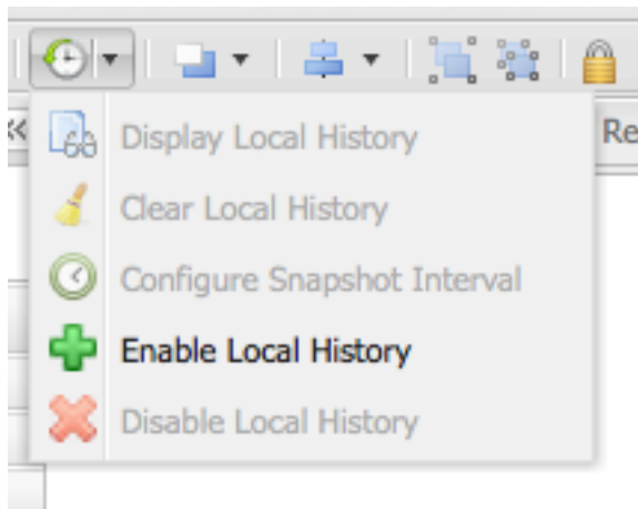
Figure 13.10. Local History
