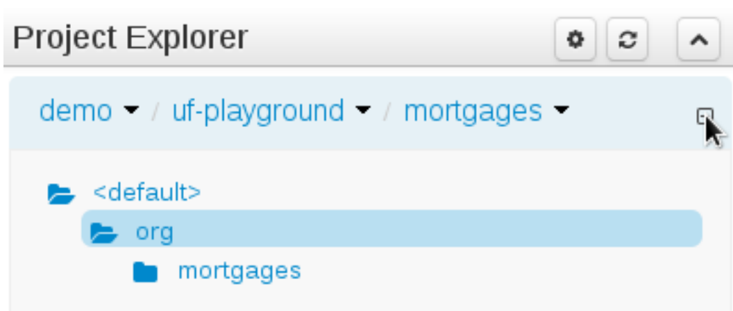
Figure 10.36. Showing packages
