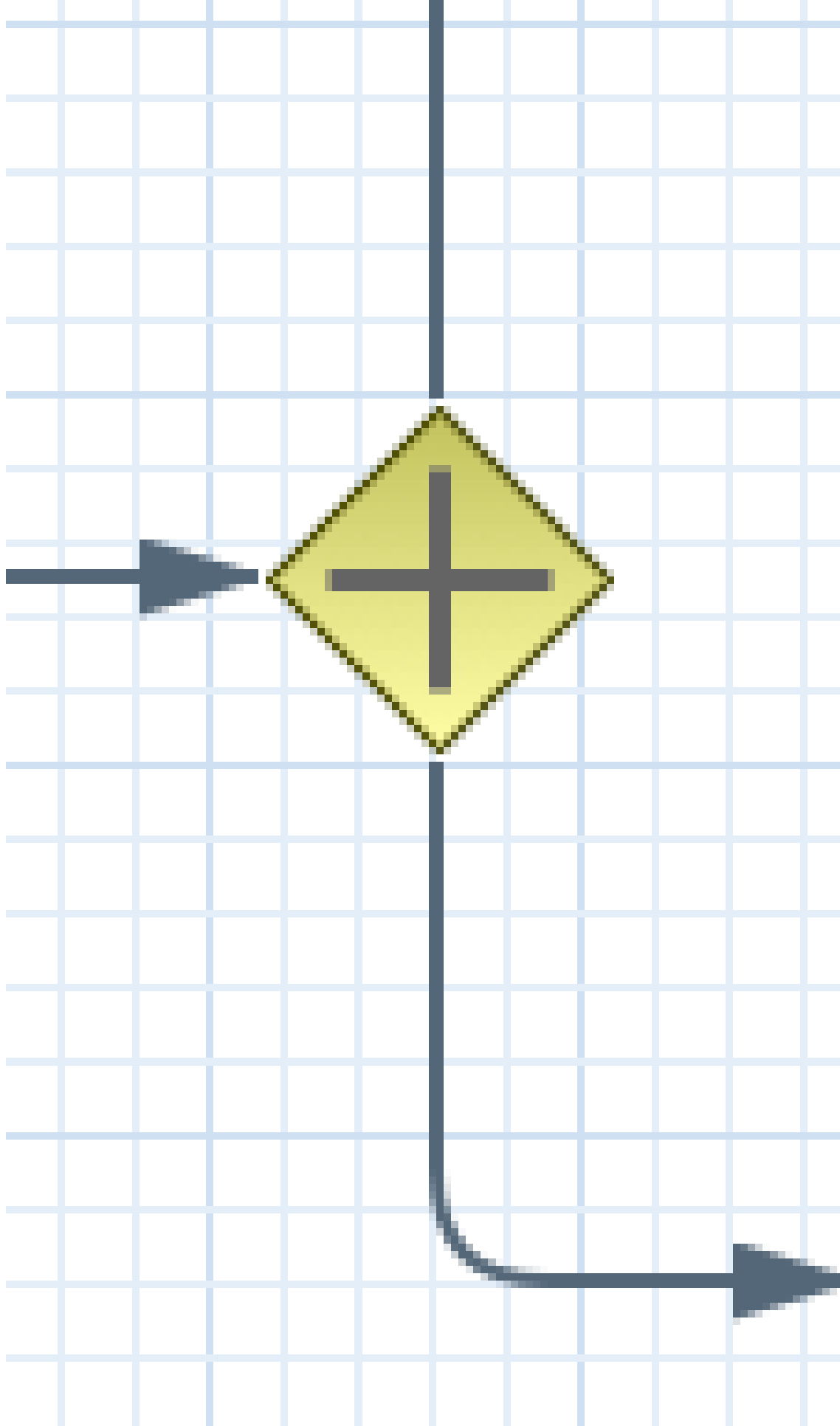
Figure 7.19. Diverging gateway
