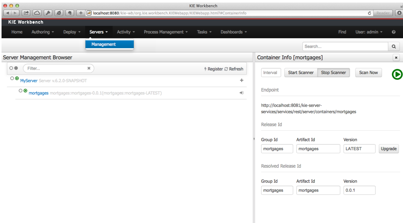
Figure 26.44. Management perspective
