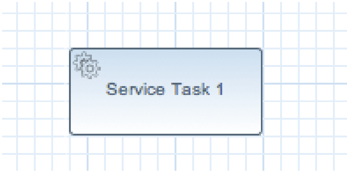
Figure 7.8. Service task
