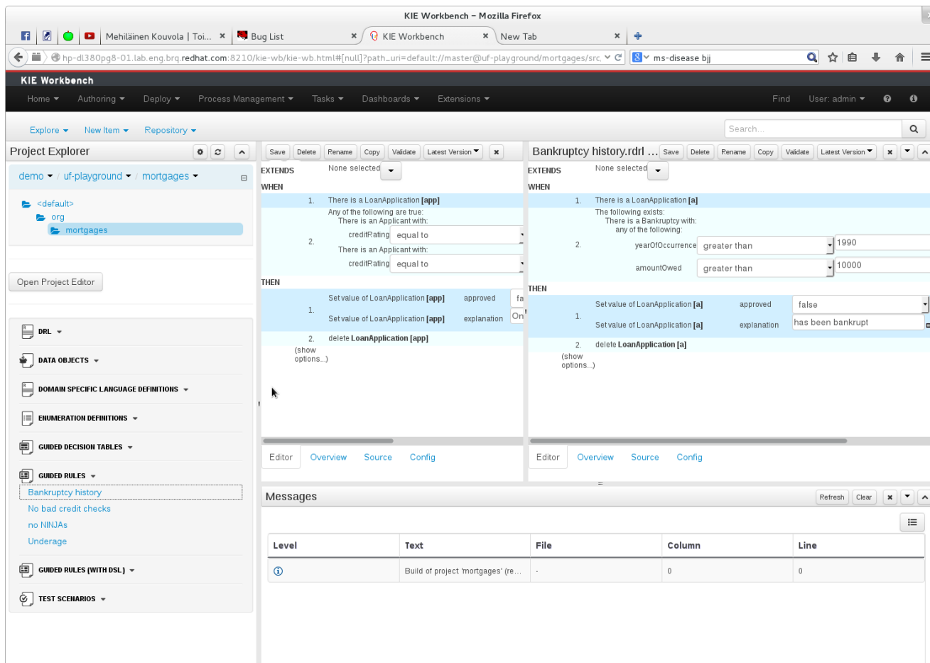
Figure 10.26. Repositioning - complete
