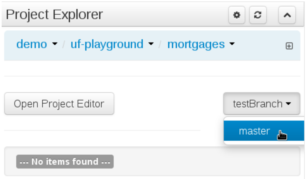
Figure 10.44. Branch selector
