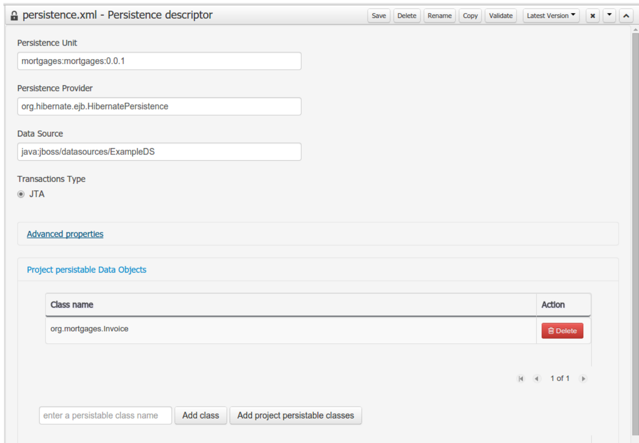
Figure 26.32. Persistence configuration
