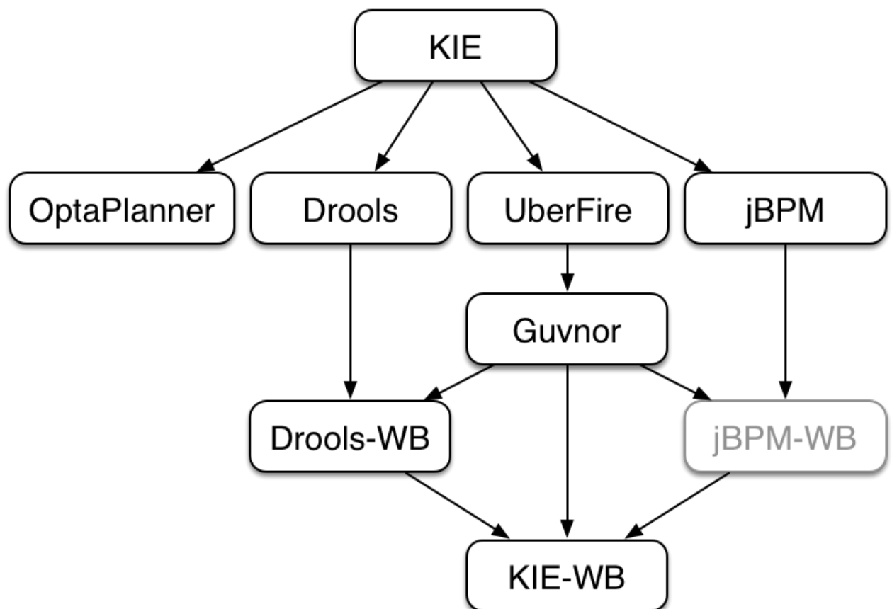
Figure 26.58. KIE Anatomy
