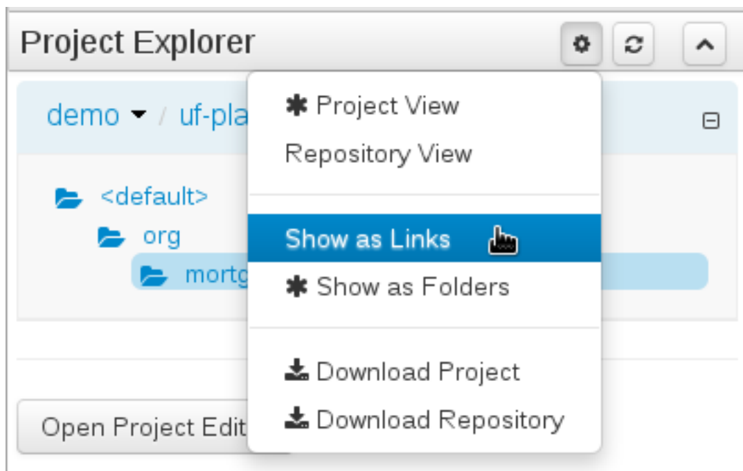
Figure 10.38. Switching view
