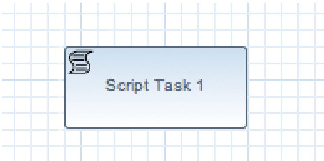
Figure 7.7. Script task
