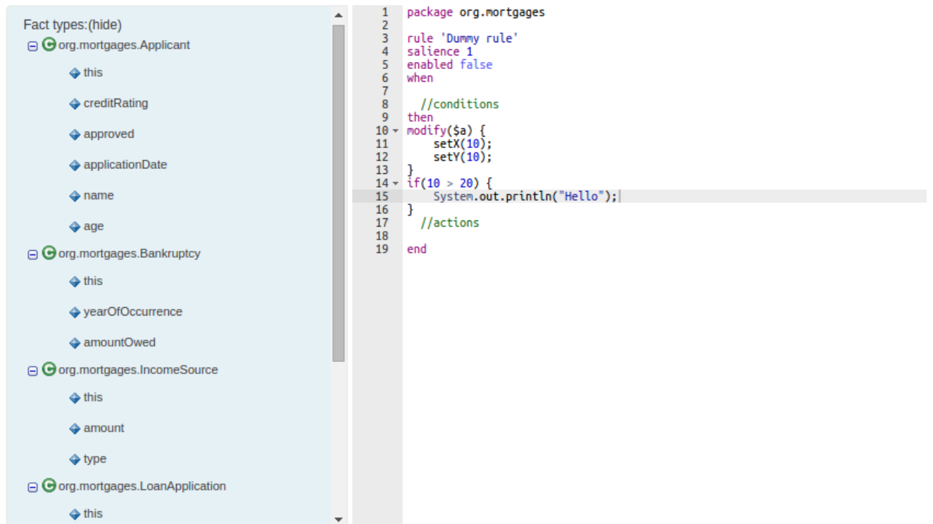
Figure 26.23. ACE Editor
