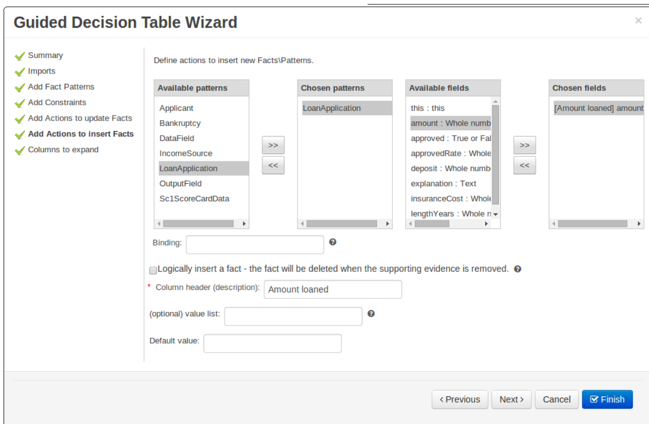
Figure 26.37. New Wizard Framework
