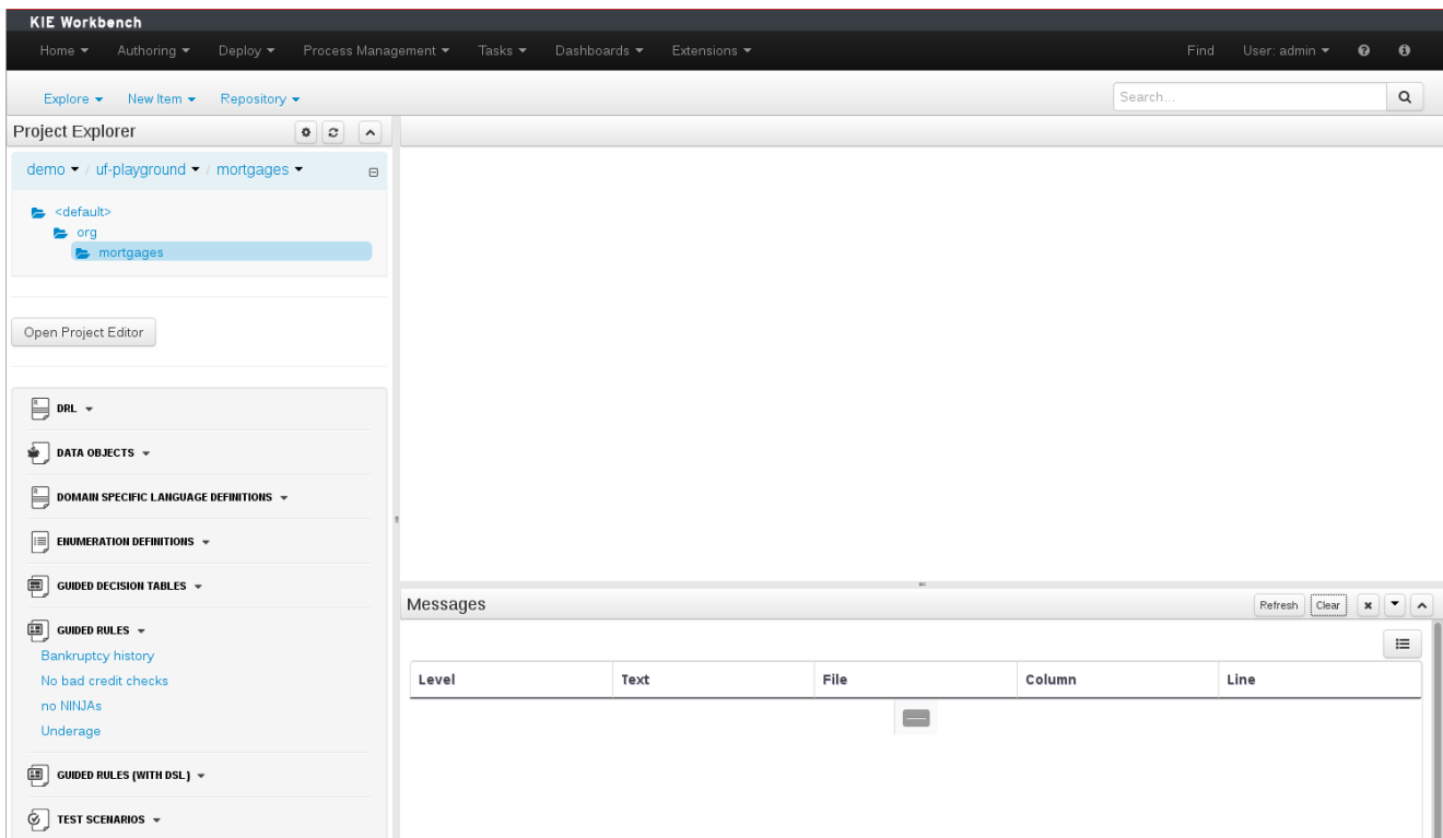
Figure 10.23. The Workbench
