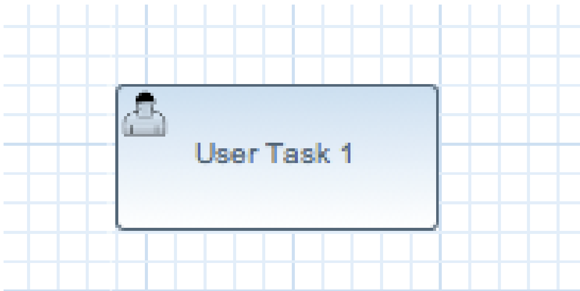
Figure 7.9. User task
