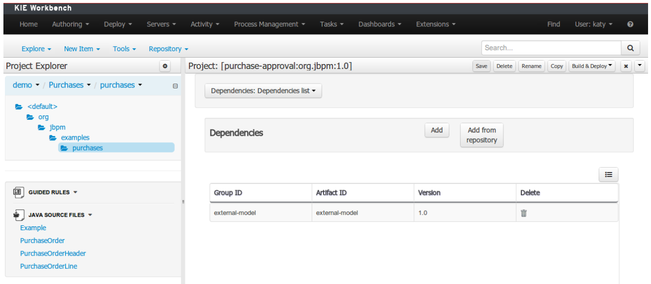
Figure 10.93. Save project.
