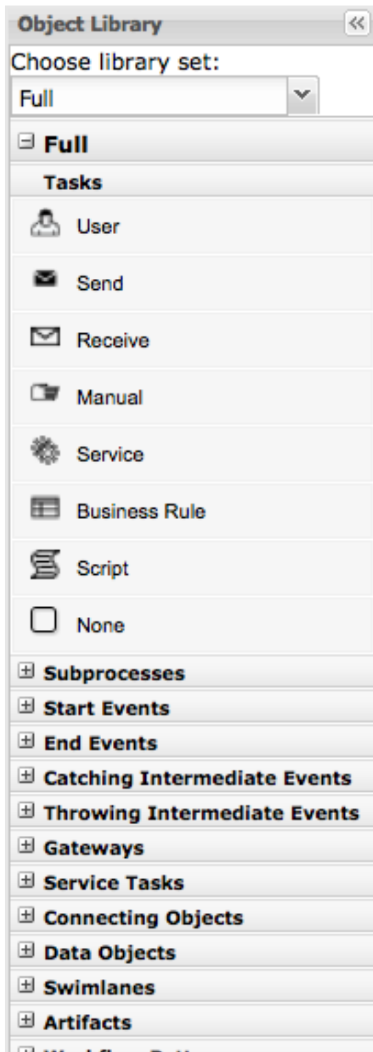
Figure 13.3. Object Repository
