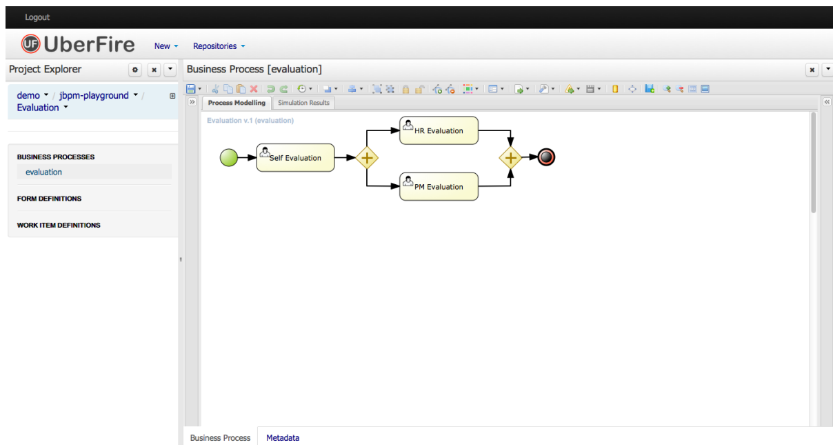
Figure 13.1. Designer
