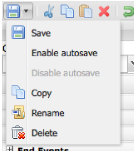
Figure 13.9. Save Button
