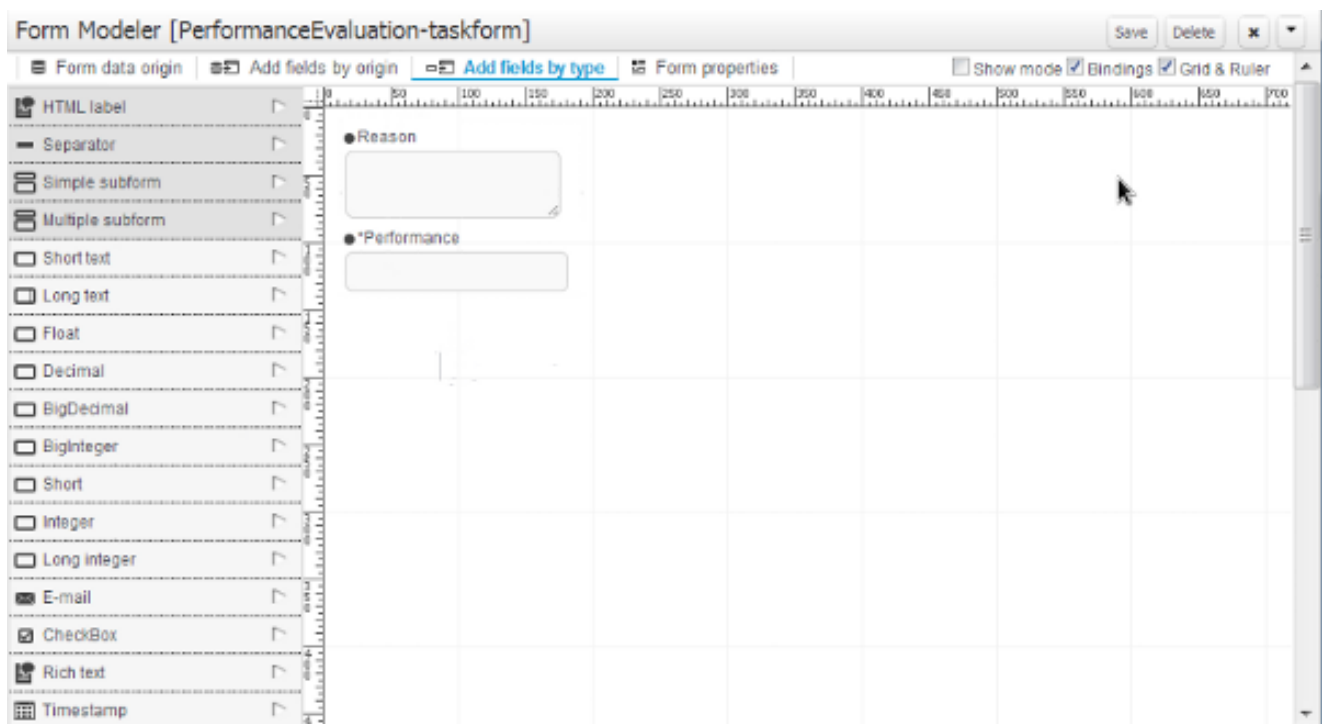
Figure 1.3. Form Modeler
