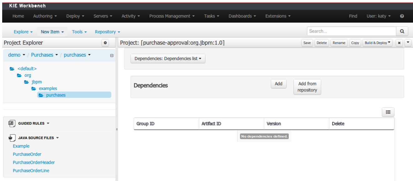
Figure 9.86. Project editor.
