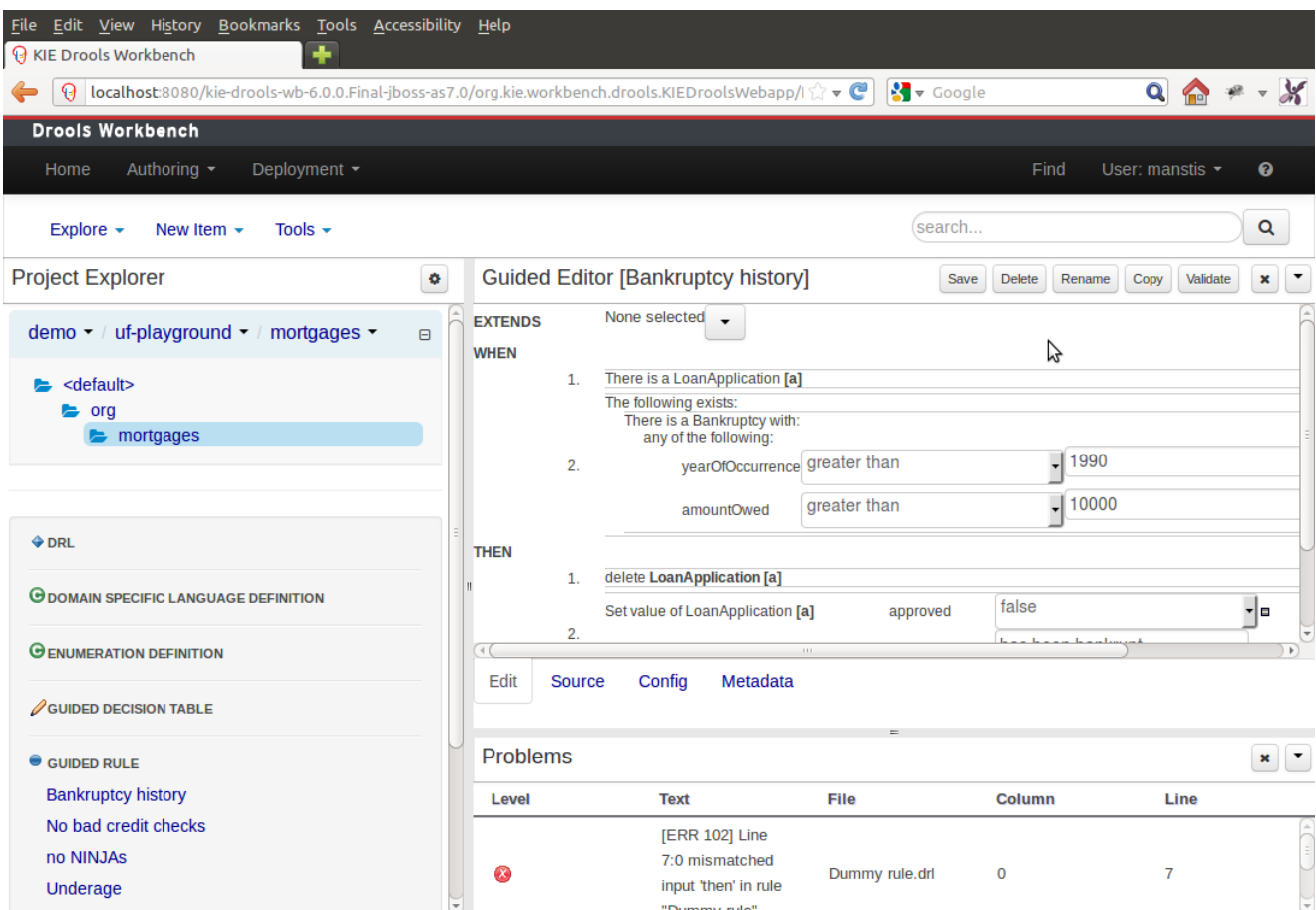
Figure 25.61. Workbench
