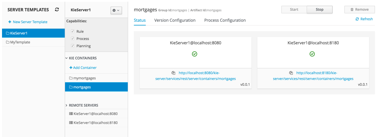
Figure 9.153. Status Container
