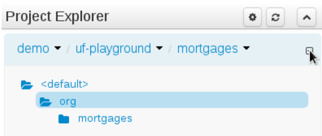
Figure 9.32. Showing packages
