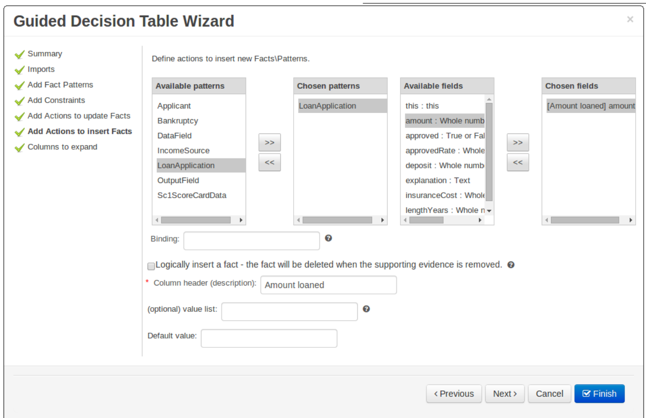
Figure 25.37. New Wizard Framework
