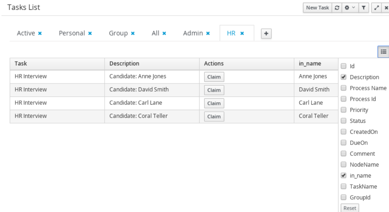
Figure 25.4. task list with task name restriction applied
