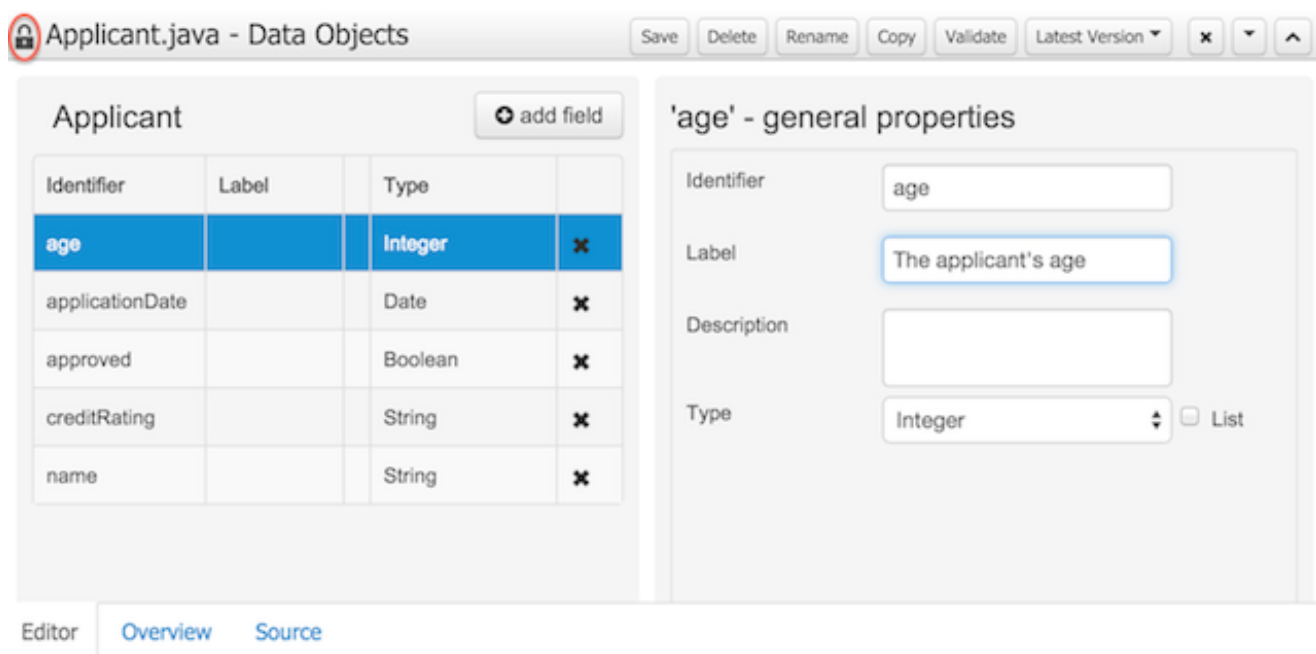
Figure 25.24. Editing an asset automatically acquires a lock
