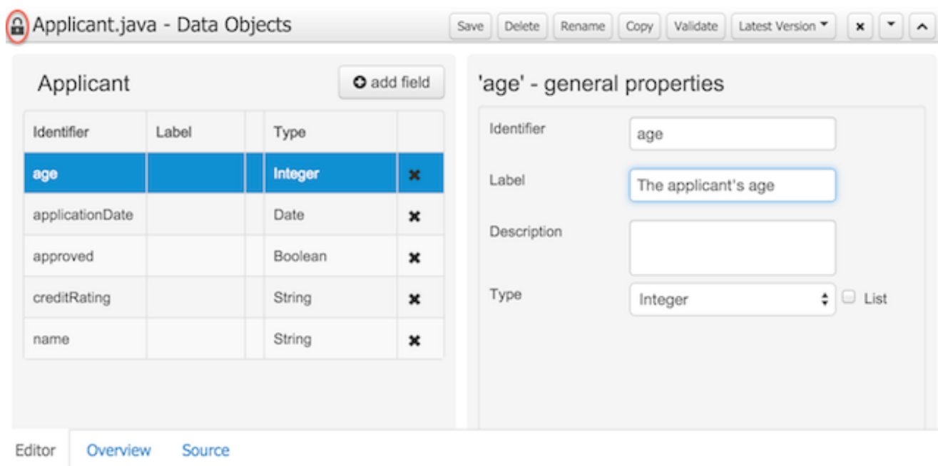
Figure 25.18. Editing an asset automatically acquires a lock
