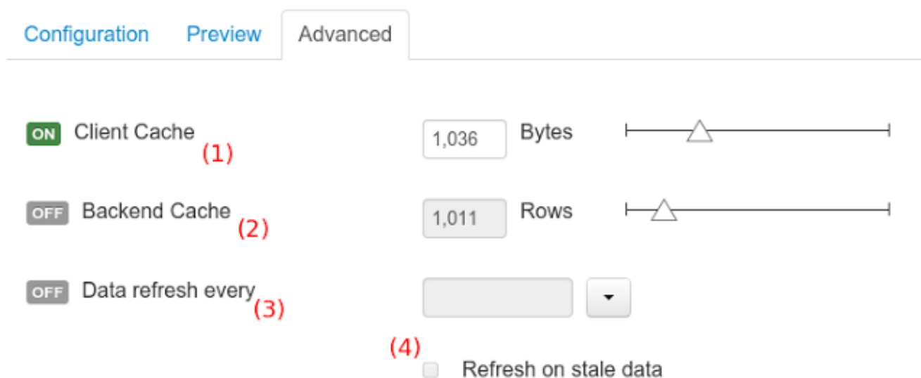
Figure 9.111. Advanced settings
