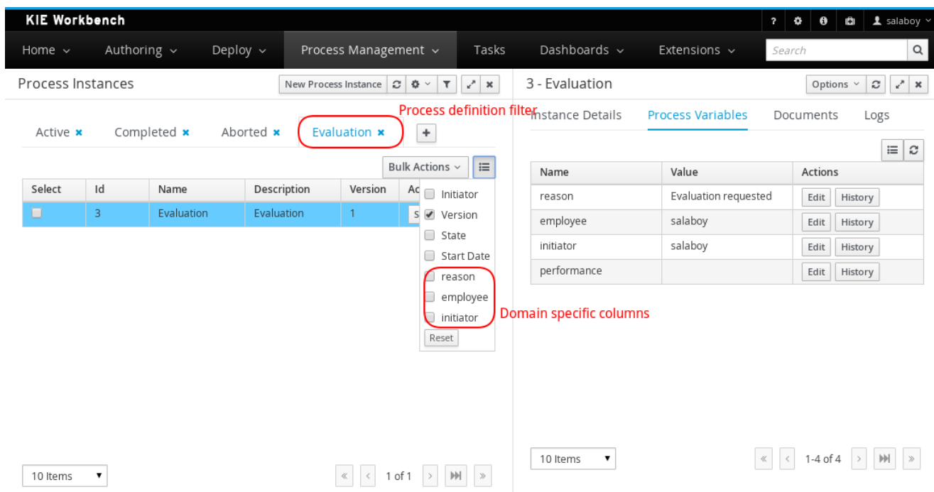
Figure 25.16.
