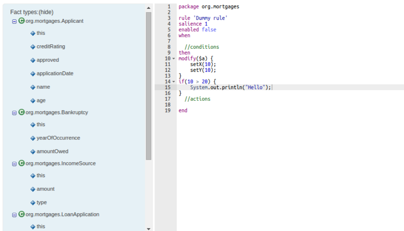
Figure 25.17. ACE Editor
