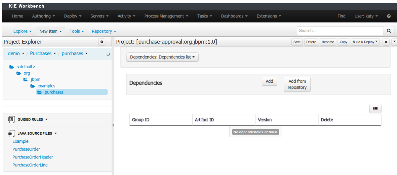
Figure 9.85. Project editor.
