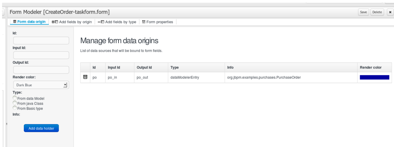
Figure 13.10. Generated form
