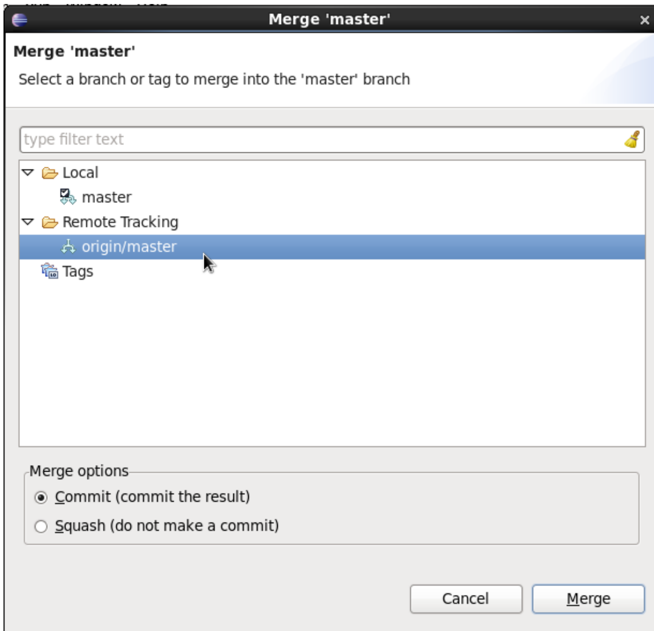
Figure 18.11.
