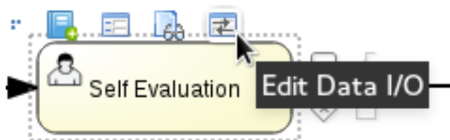
Figure 25.12.
