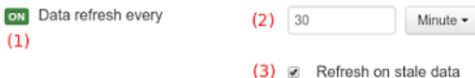
Figure 9.113. Refresh settings
