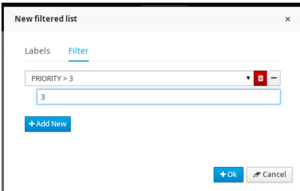
Figure 25.14.
