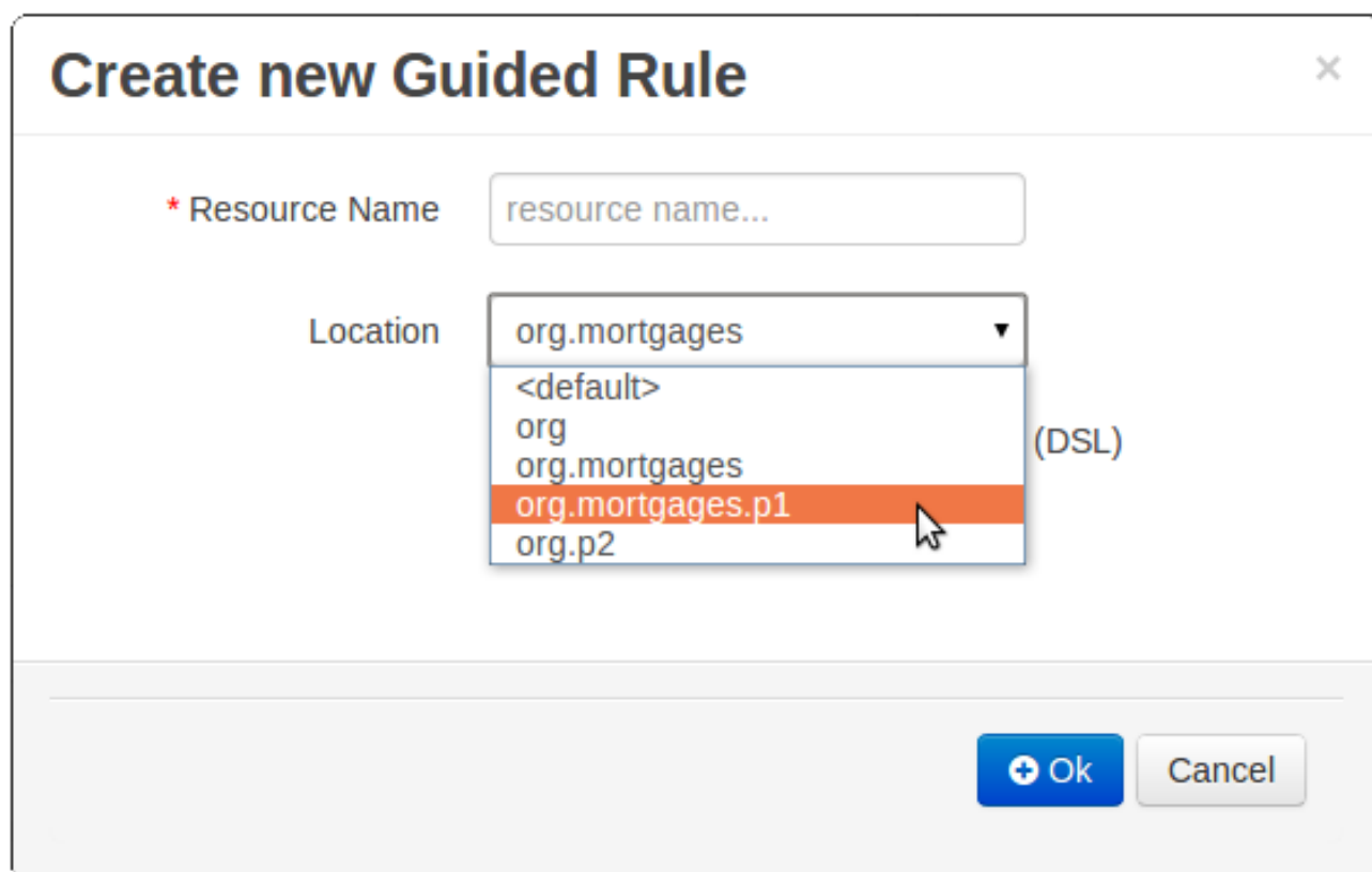
Figure 25.43. Package selector
