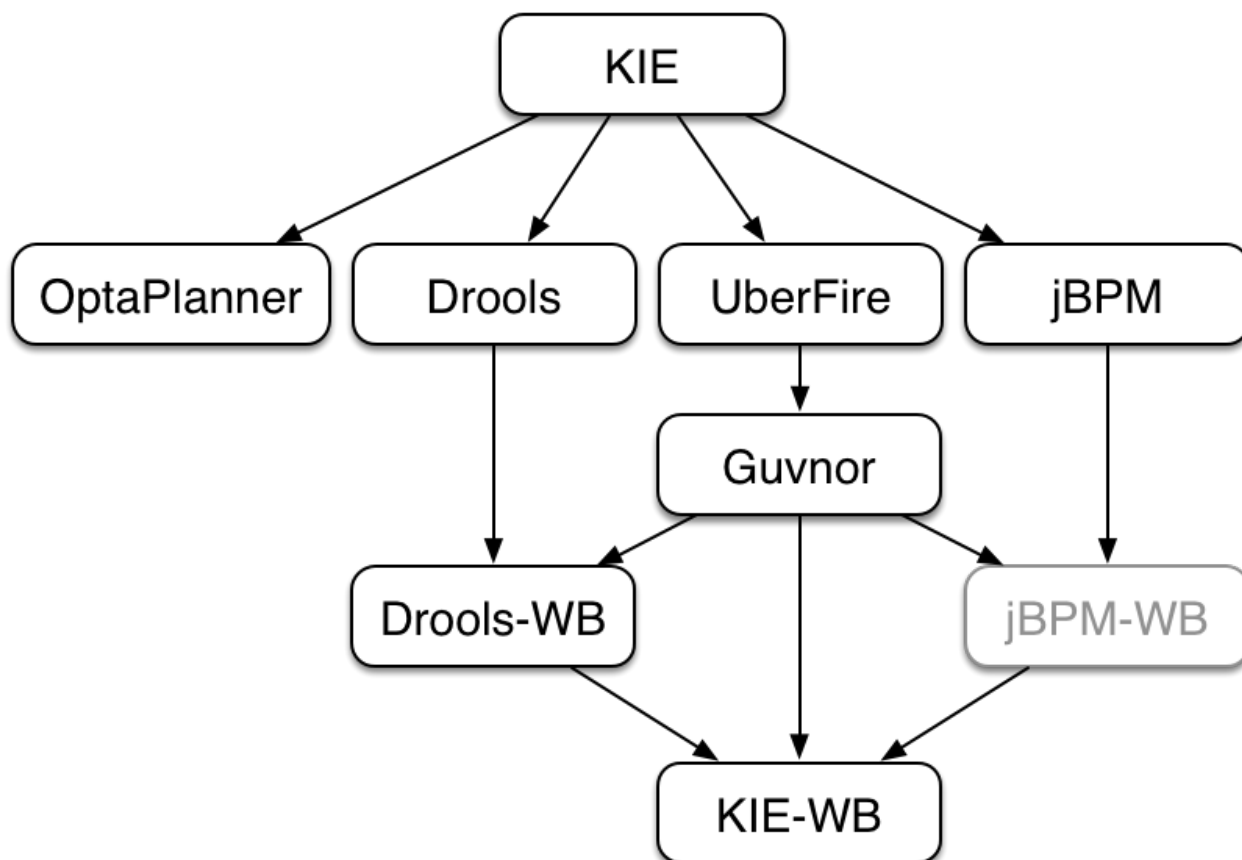
Figure 25.52. KIE Anatomy
