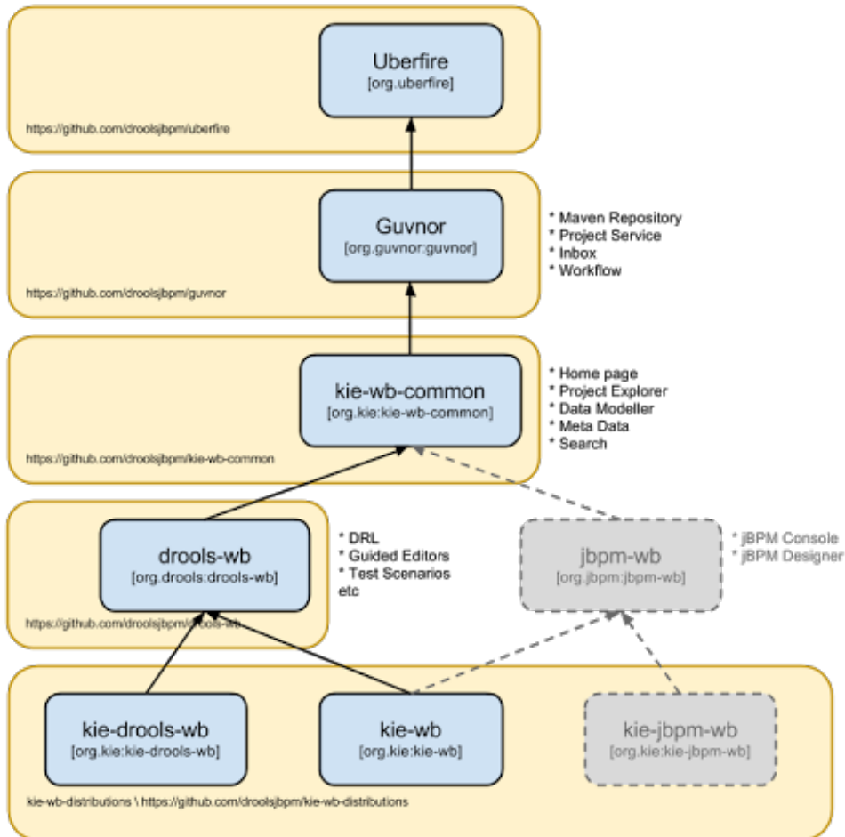
Figure 25.54. Module Structure
