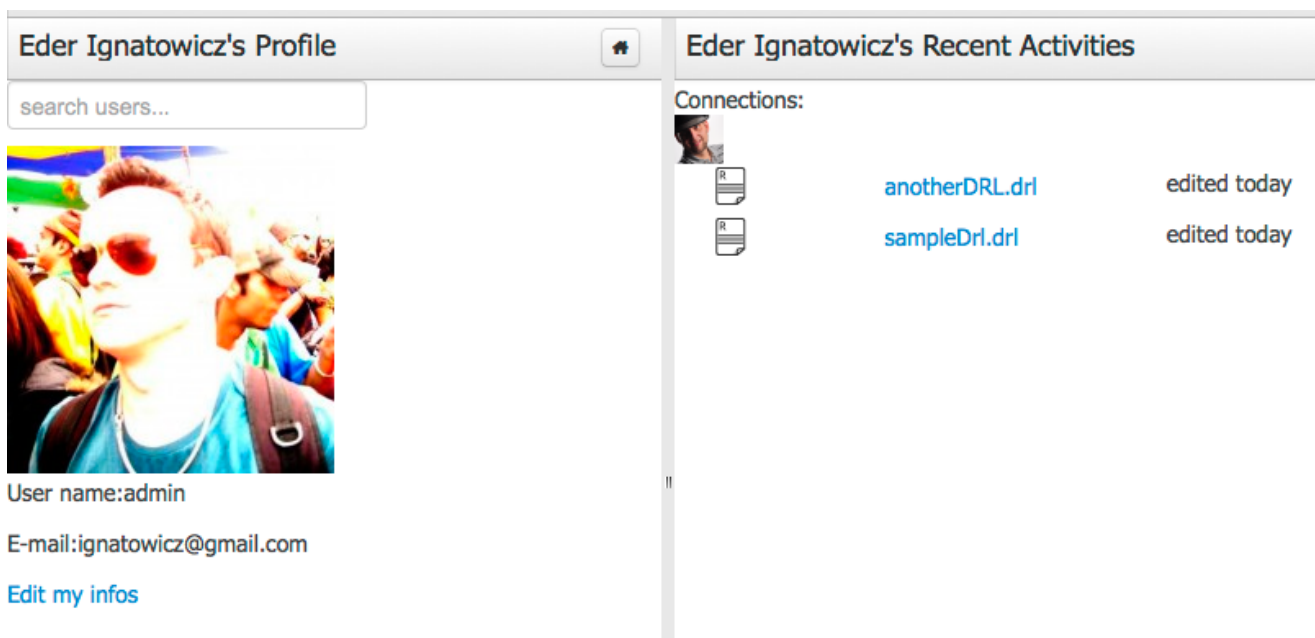
Figure 25.36. People Perspective
