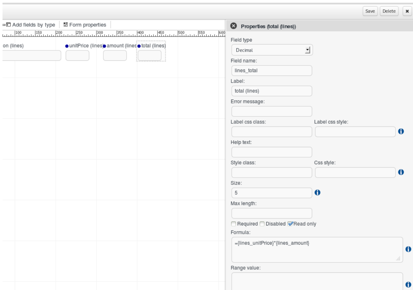
Figure 13.26. Configuring formulas
