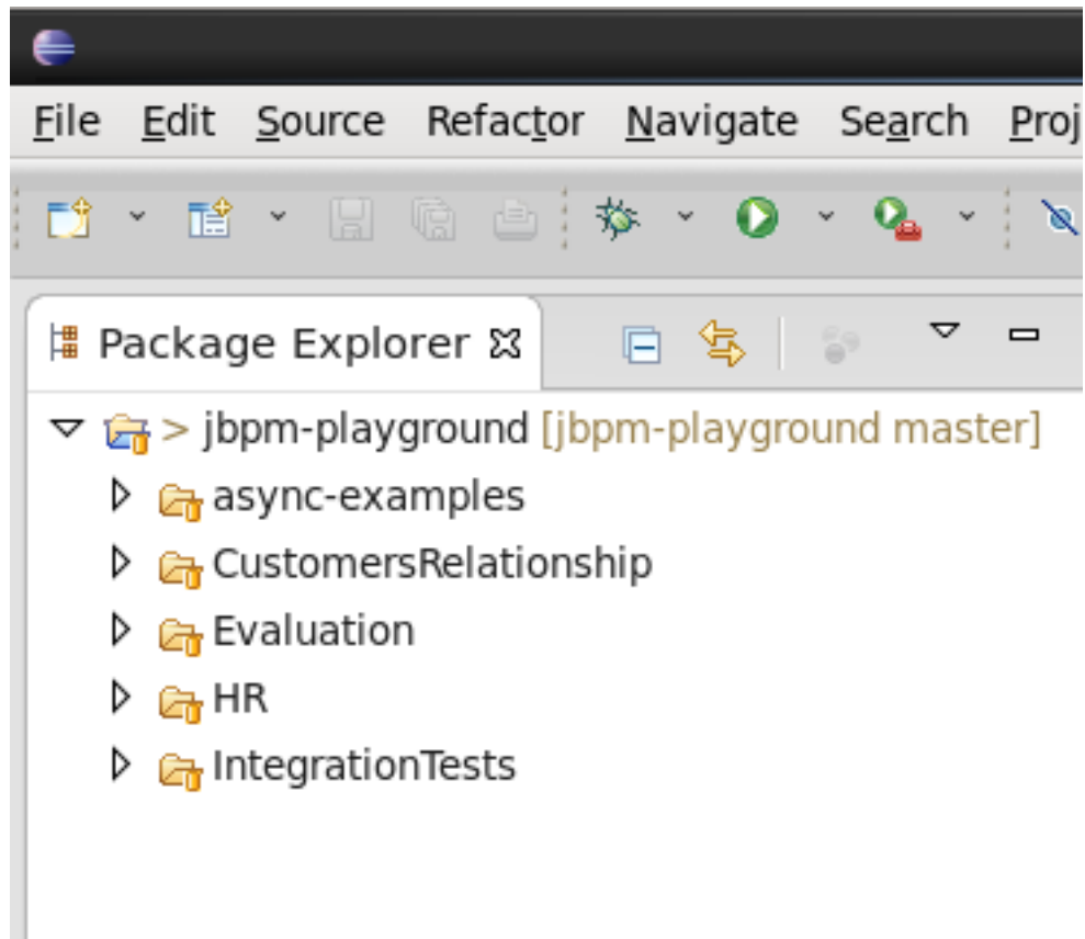
Figure 18.9.
