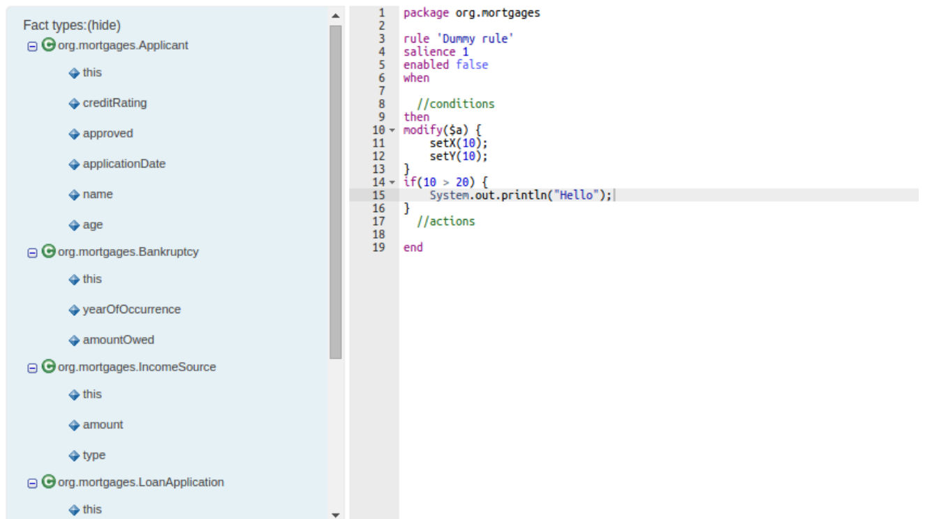
Figure 25.13. ACE Editor
