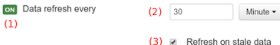
Figure 9.110. Refresh settings
