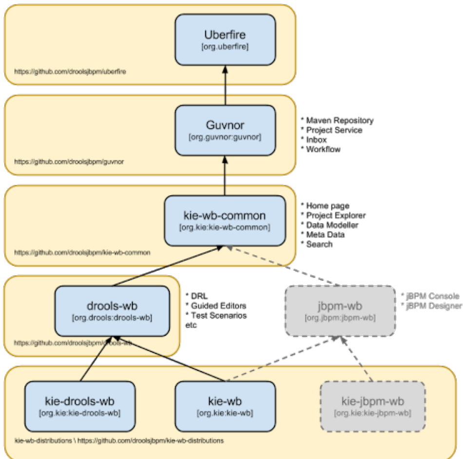
Figure 25.50. Module Structure
