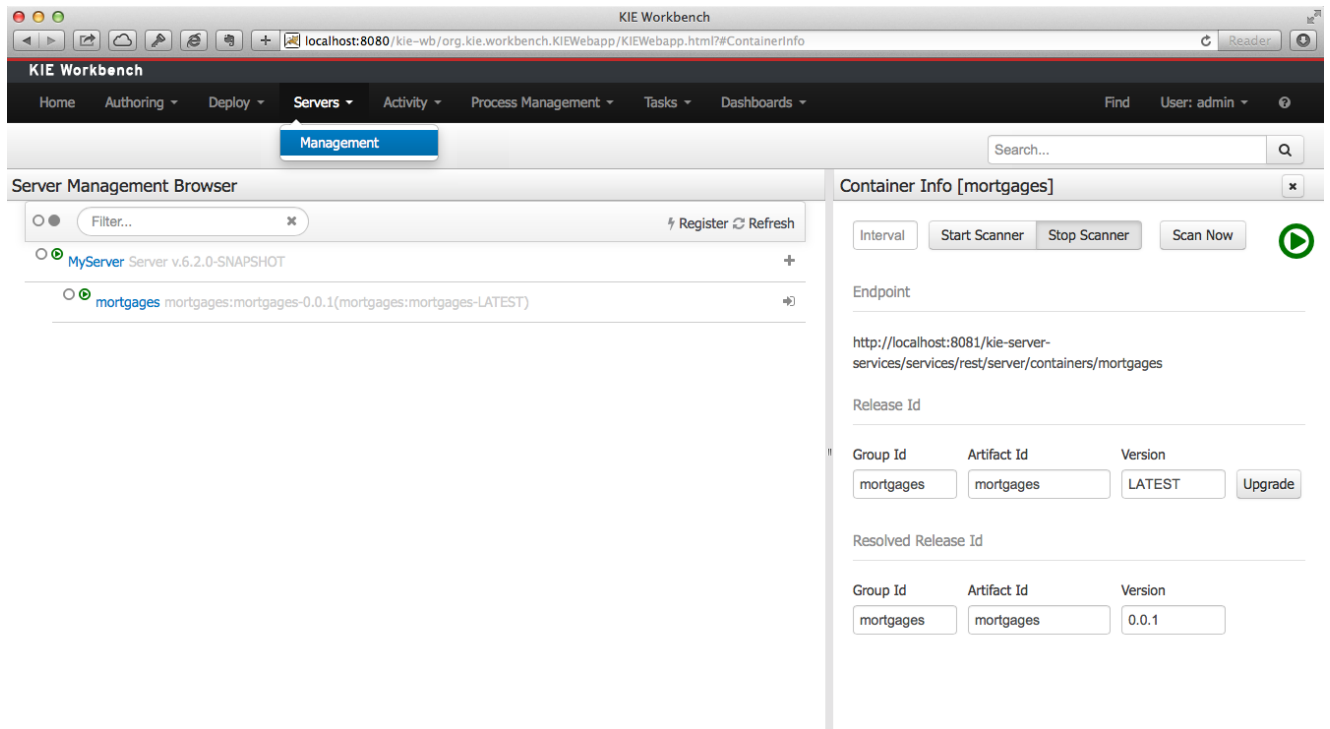
Figure 25.34. Management perspective
