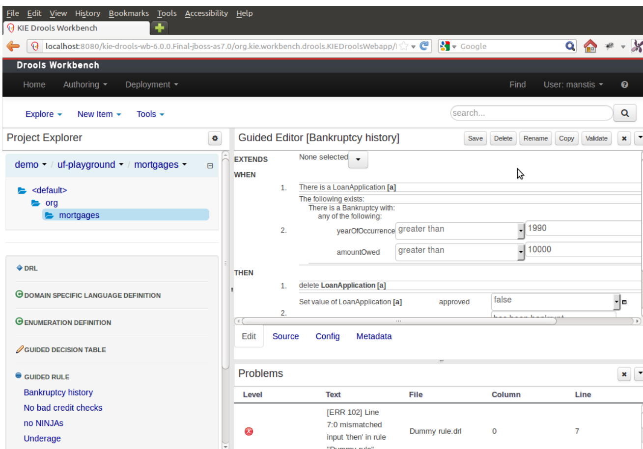
Figure 25.49. Workbench
