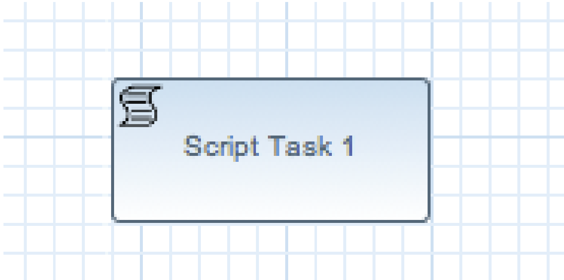
Figure 6.7. Script task
