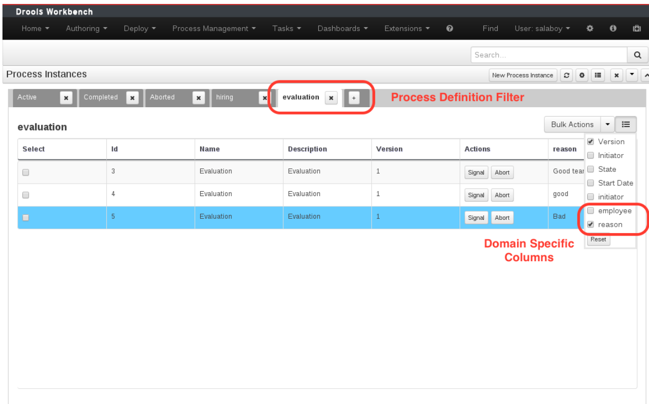
Figure 25.12.
