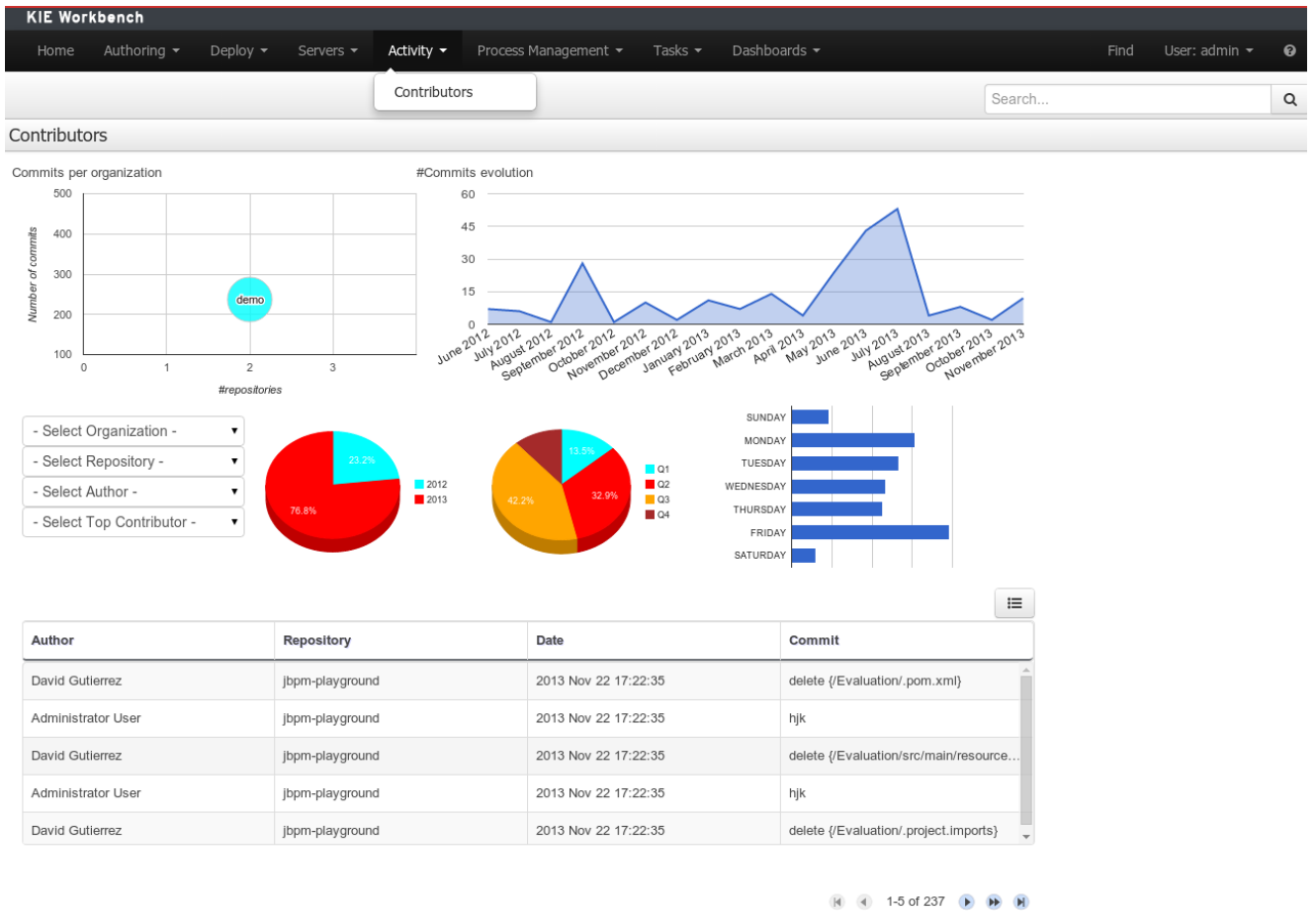
Figure 25.38. Contributors perspective
