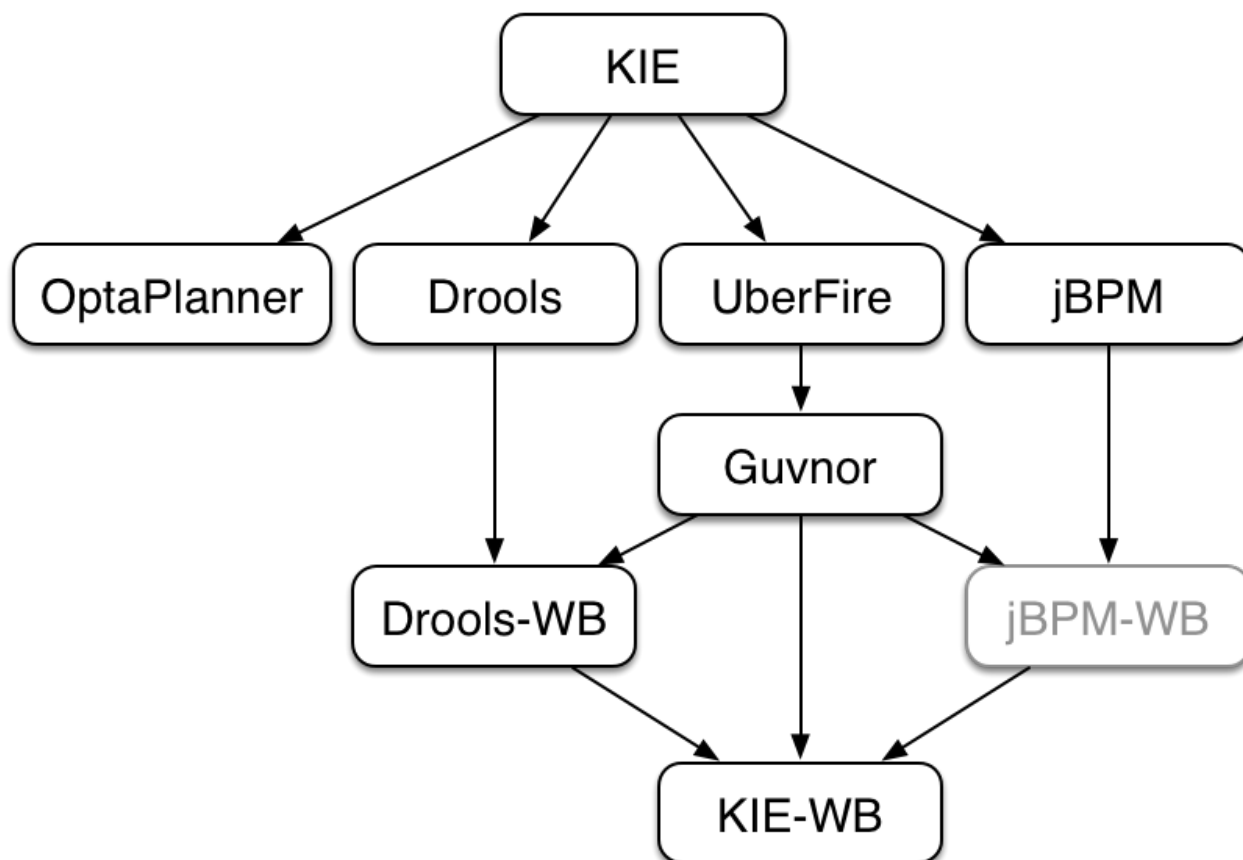
Figure 25.48. KIE Anatomy
